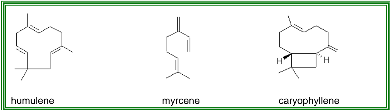
Fig. 1: Characteristic hop oil compounds
